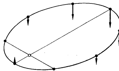
Fig. 4 Optimum thrust program for change in \theta_2 ( e = 0.707 ).
