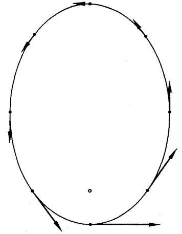
Fig. 1 Optimum thrust program for change in a ( e = 0.707 ).
